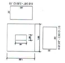
SAPATAS - S1, S2, S3, S4, S5, S6, S7, S8, S9, S11, S12, S13, S14, S15, S16, S17, S18 PLANTA E CORTE - ESC. 1/25
